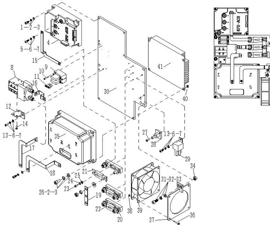
Fig. 21 Controller Assembly
