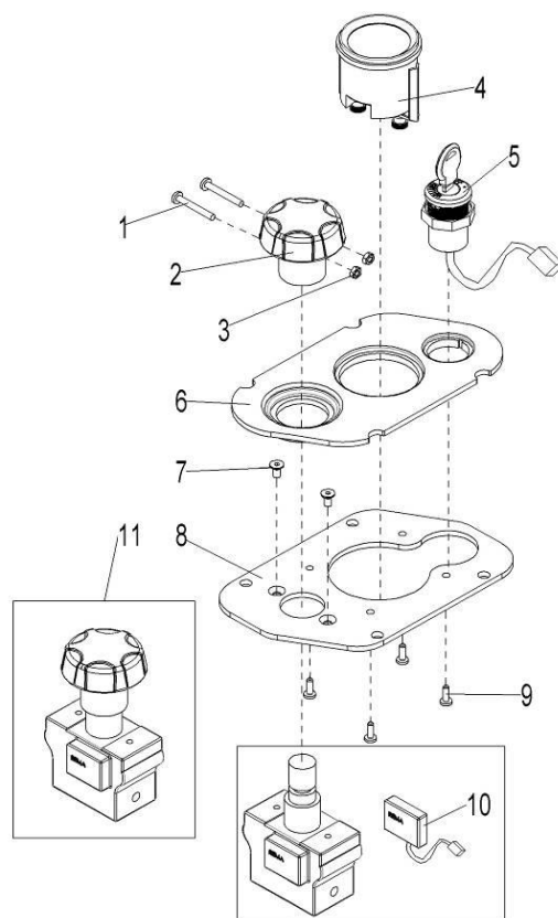
Fig.10 Indicator assembly
