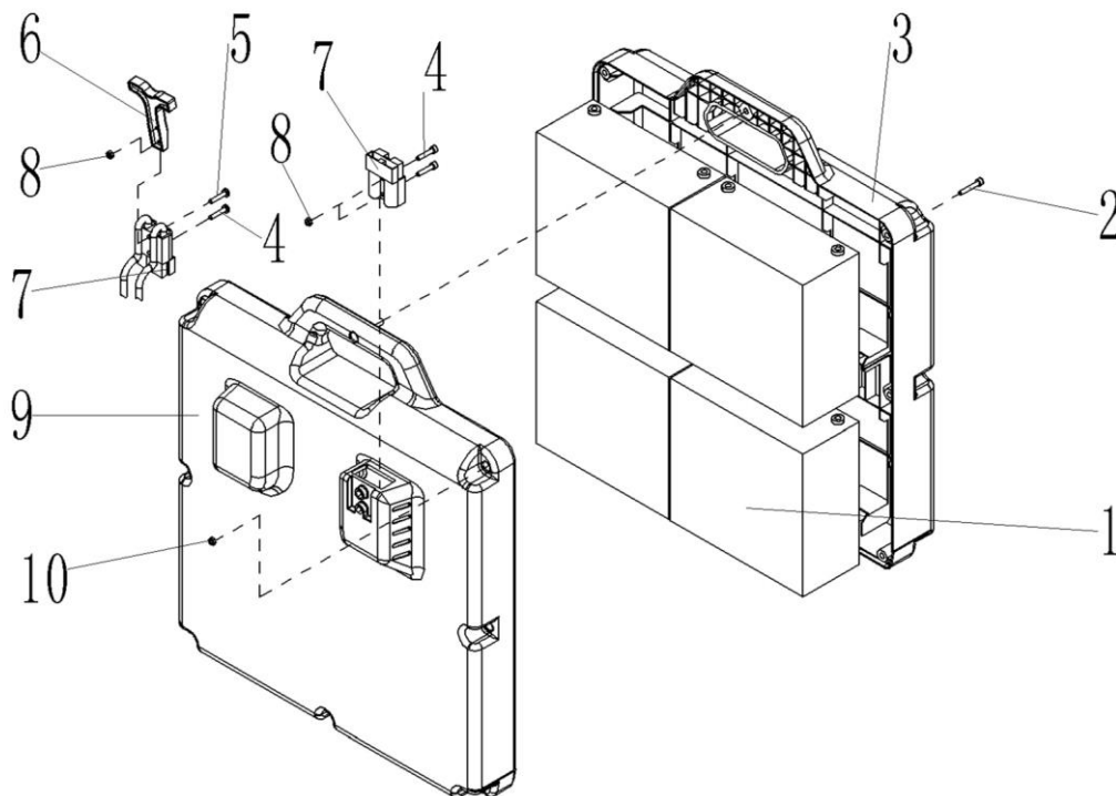
Fig.13 Power supply assembly
