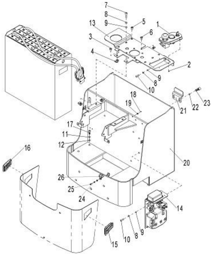
Fig. 8 Truck body
