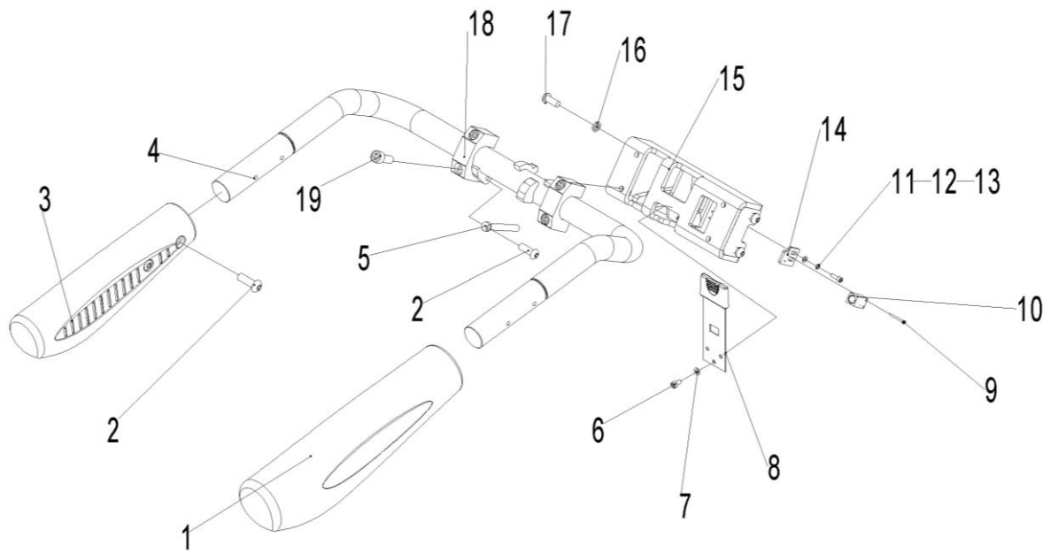
Fig. 31 Protective arm
