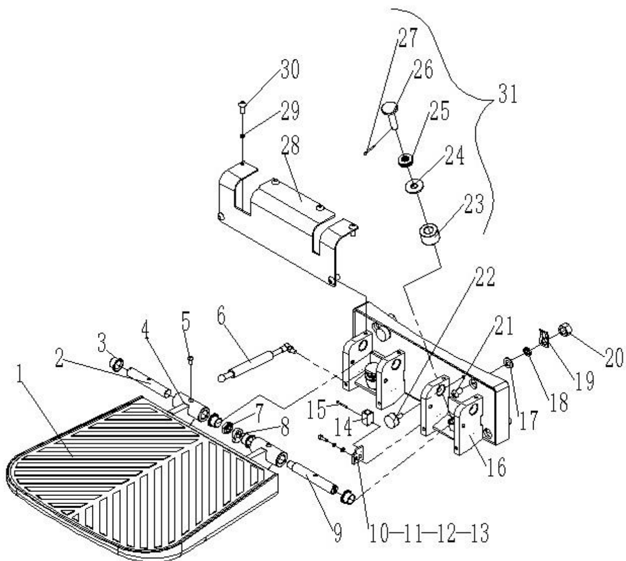
Fig. 30 Foldable platform
