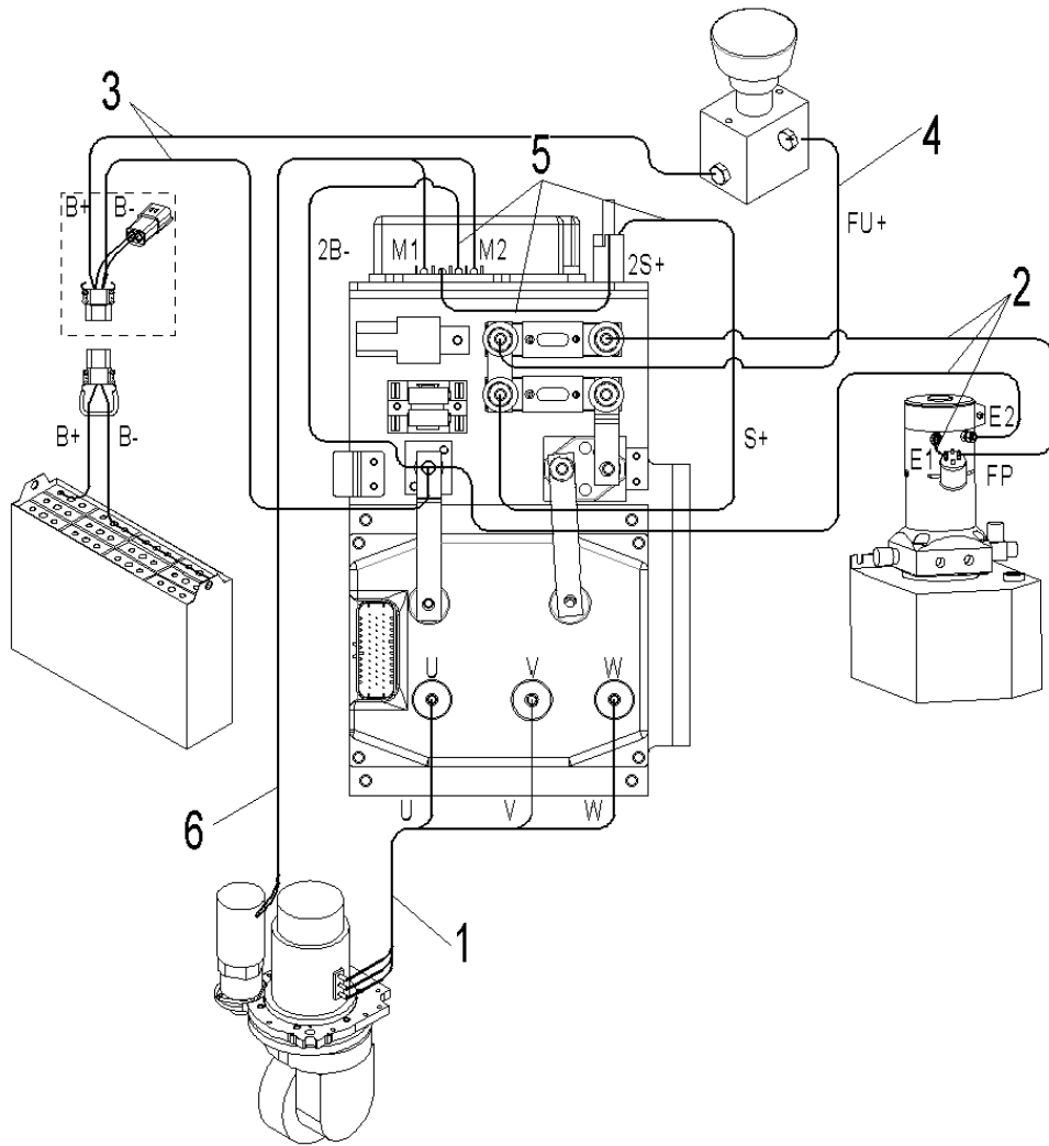
Fig. 25 Main circuit wiring (Electrical steering)
