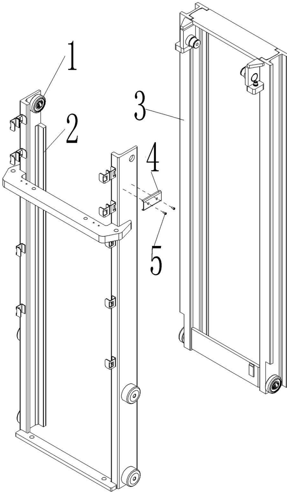
Fig. 12 Mast system
