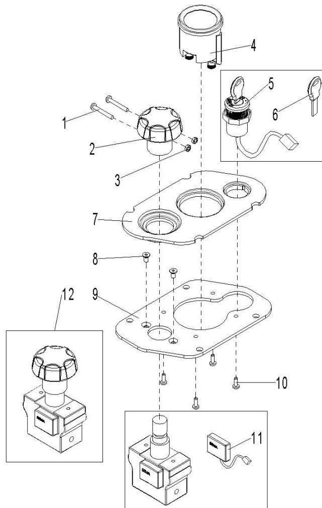
Fig. 10 Instrument assembly
