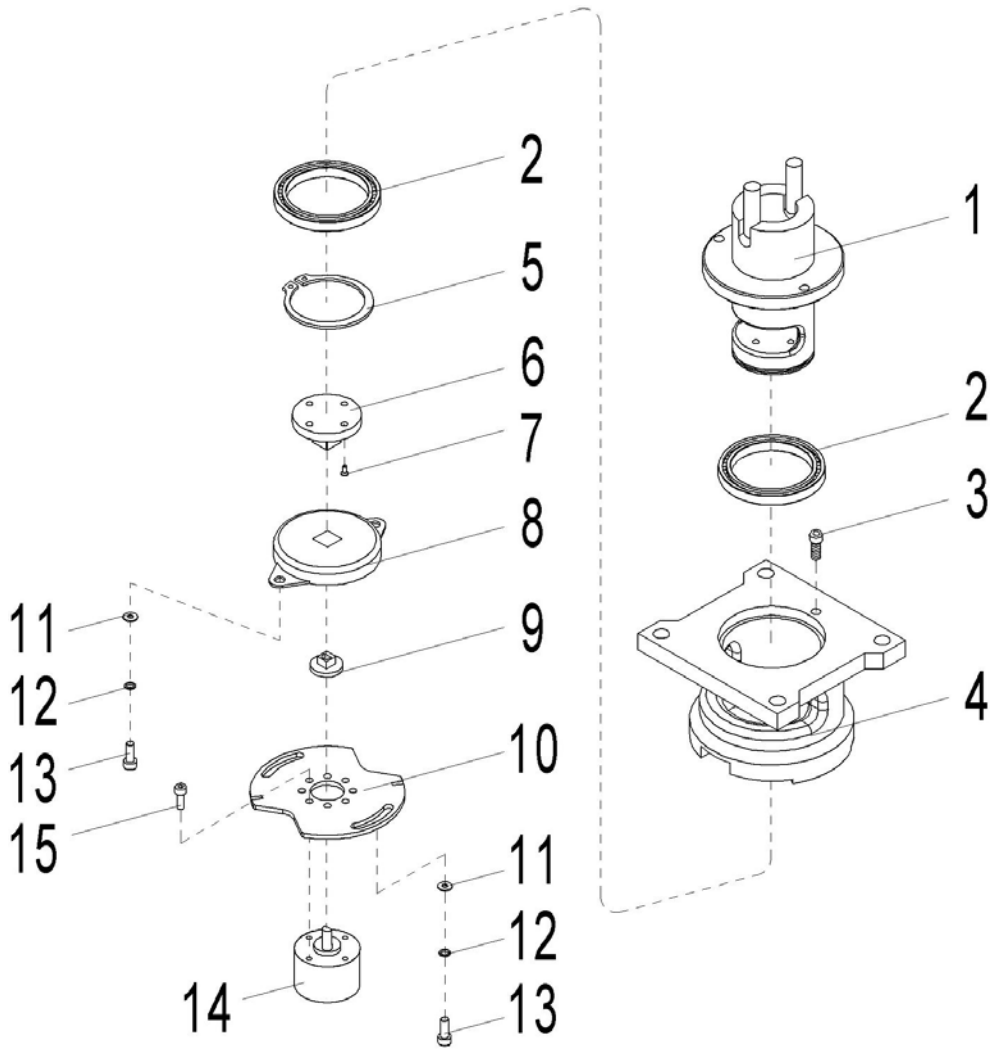
Fig. 23 EPS components
