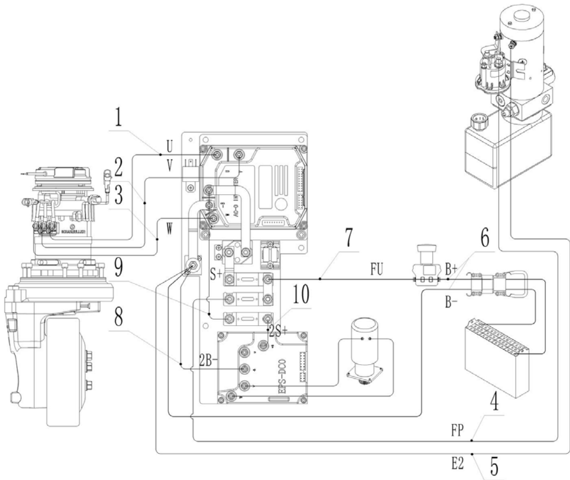
Fig. 34 Main Circuit (EPS)
