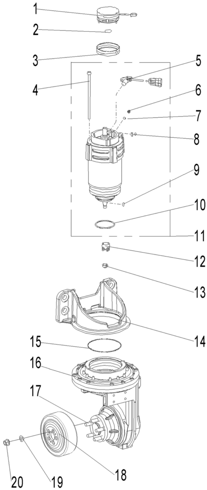
Fig. 6 Driving assembly (Manual steering)
