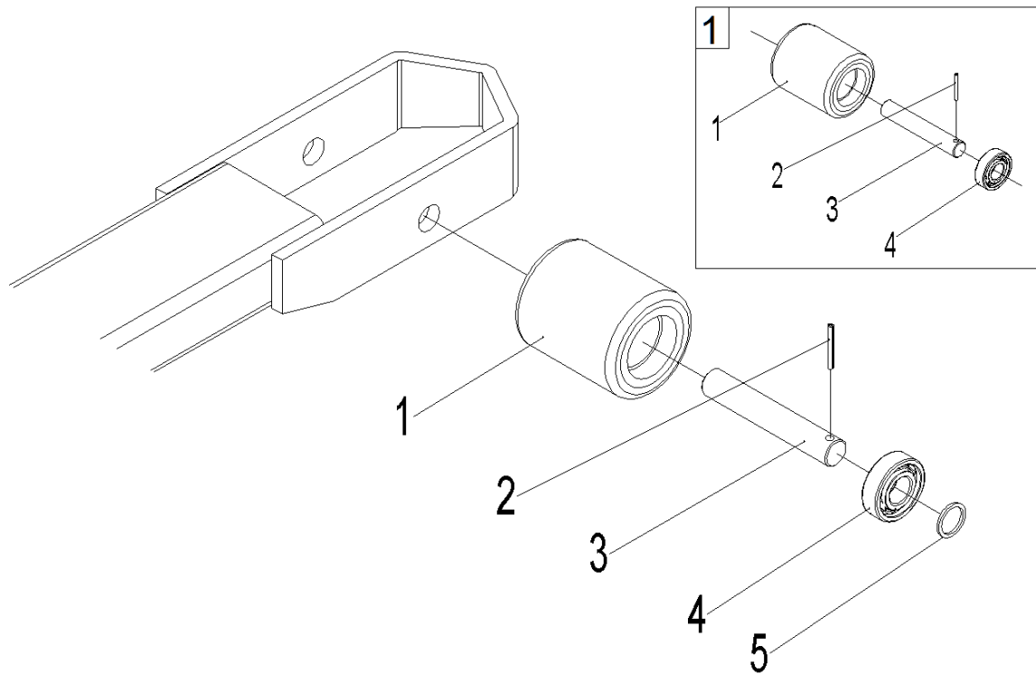
Fig. 7 Load wheel
