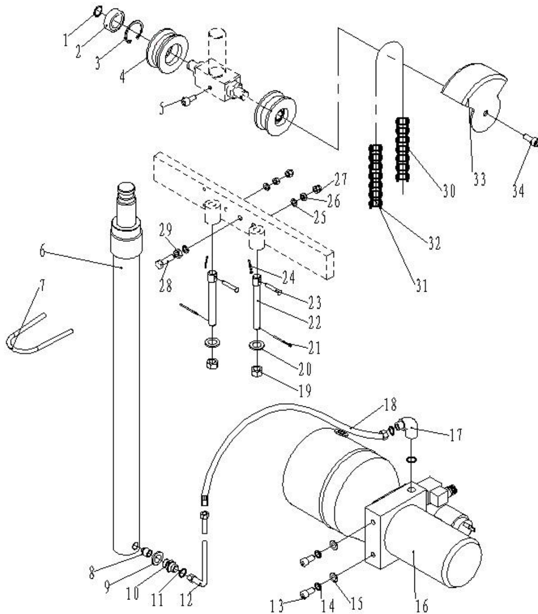
12.2 Two-stage-mast hydraulic system
