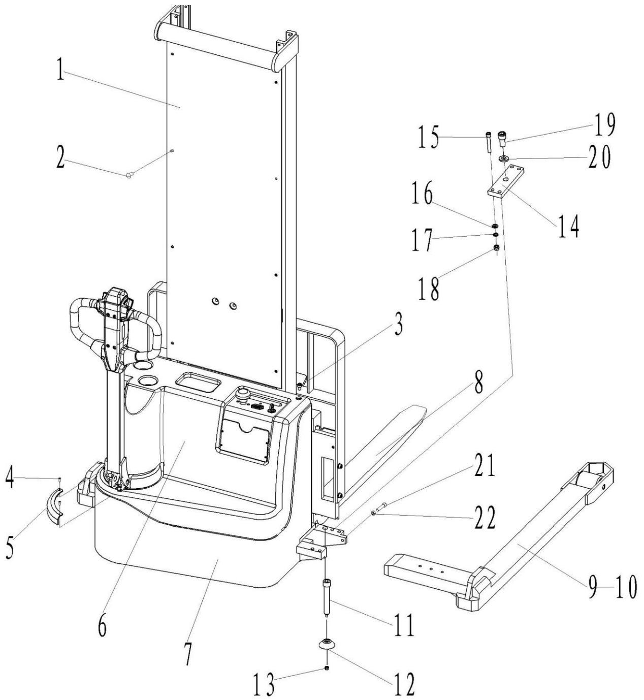
Fig. 3 Appearance
