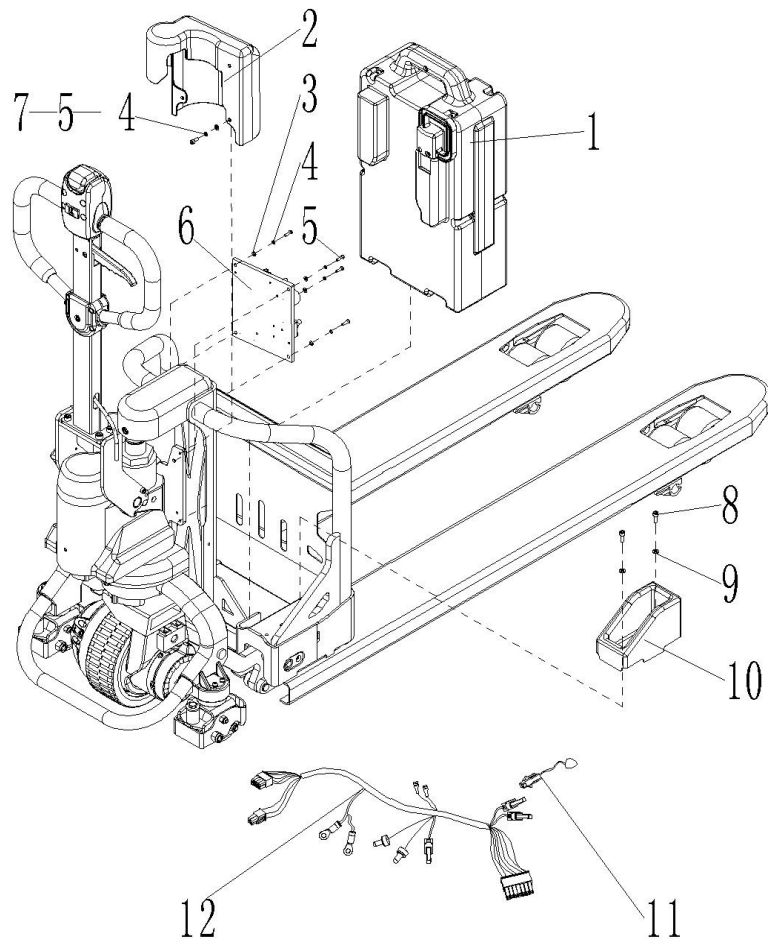
Fig. 9 Truck Parts
