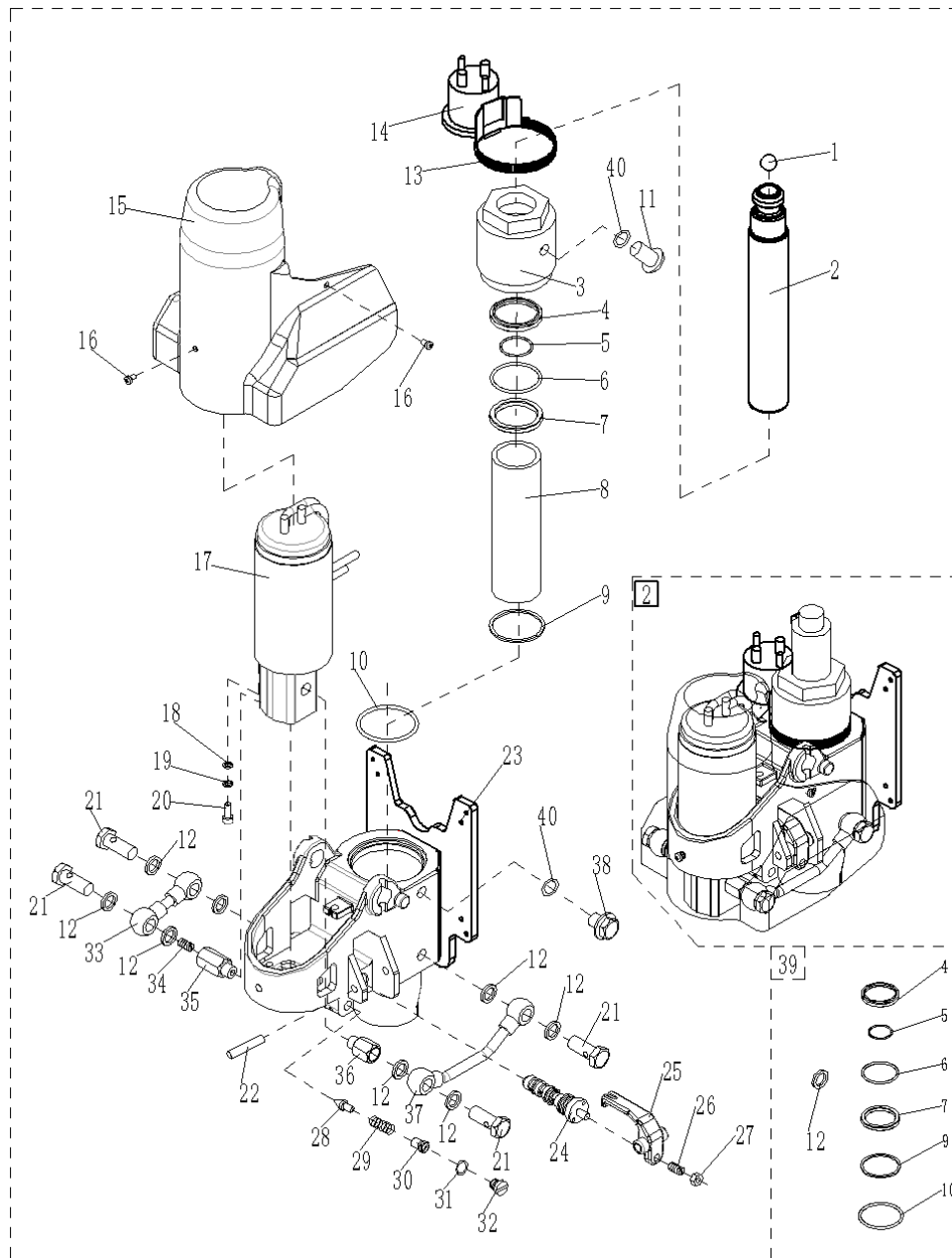
Fig. 5 Hydraulic Parts
